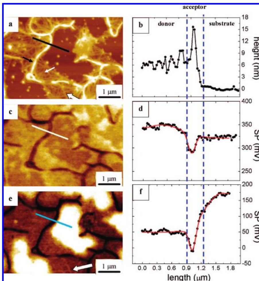
Figure 5. KPFM data on thin films of P3HT and P-PDI. (a) AFM topography image of an ultrathin blend of P-PDI and P3HT deposited on silicon. (c, e) SP images of the same area as in (a), under (c) no illumination and (e) illumination with white light ( \sim 60 \text{ mW cm}^{-2} ). An overall negative potential shift upon light illumination is known to occur in these types of KPFM measurements, as previously reported for thick layers (see the text); this is the reason why both PDI and P3HT appear more negative (darker) than the exposed bare silicon areas upon illumination. (b, d, f) Measured (black lines and circles) and simulated (red lines) profiles obtained by tracing the arbitrary lines in the corresponding images (a), (c), and (e). The SP values depicted are the measured ones and therefore differ from the calculated asymptotic true values reported in Table 1. Z ranges: (a) 32 nm, (c) 120 mV, and (e) 120 mV.
